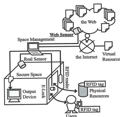
Figure 1. Spatio-temporal Web sensors in secure spaces.
