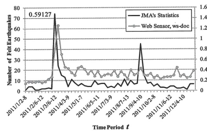
Figure 7. JMA's weekly statistics and Web Sensor's data using Web documents searched by Google for earthquake in Hokkaido prefecture, 2011
