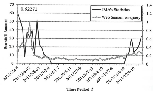
Figure 3. JMA's weekly statistics and Web Sensor's data using Web queries collected by Google Trends for snowfall in Hokkaido prefecture, 2011.
