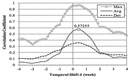
Figure 10. Dependency of temporally-shifted Web Sensor, ws\text{-}query_{\delta} , using Web queries collected by Google Trends on temporal shift \delta for earthquake.
