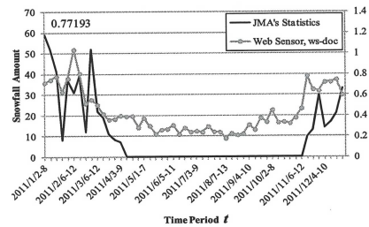
Figure 6. JMA's weekly statistics and Web Sensor's data using Web documents searched by Google for snowfall in Hokkaido prefecture, 2011
