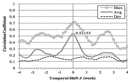
Figure 11. Dependency of temporally-shifted Web Sensor, ws\text{-}doc_{\delta} , using Weblog documents searched by Google on temporal shift \delta for rainfall.
