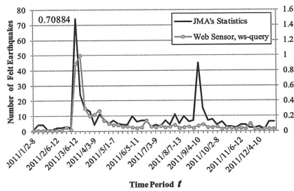
Figure 4. JMA's weekly statistics and Web Sensor's data using Web queries collected by Google Trends for earthquake in Hokkaido prefecture, 2011.
