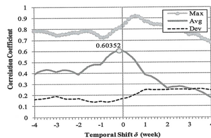
Figure 9. Dependency of temporally-shifted Web Sensor, ws-query δ , using Web queries collected by Google Trends on temporal shift δ for snowfall.
