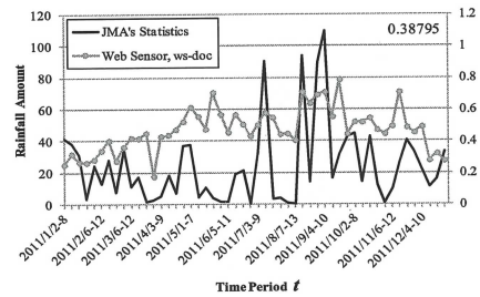
Figure 5. JMA's weekly statistics and Web Sensor's data using Web documents searched by Google for rainfall in Hokkaido prefecture, 2011.
