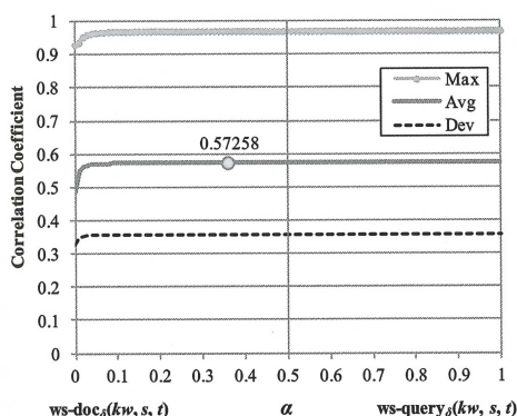
Figure 19. Dependency of combined Web Sensor, ws_{\delta}^{\alpha} , using Web queries and Weblog documents on combination parameter \alpha for earthquake.
