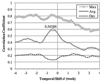
Figure 12. Dependency of temporally-shifted Web Sensor, ws\text{-}doc_{\delta} , using Weblog documents searched by Google on temporal shift \delta for snowfall.
