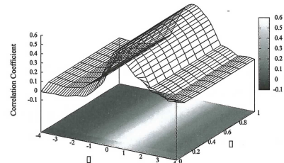
Figure 16. Dependency of combined Web Sensor, ws_{\delta}^{\alpha} , using Web queries and documents on temporal shift \delta and combination param \alpha for earthquake. ( Max 0.57258 when \delta = +0.429 (week) = +3 (day) and \alpha = 0.37330 )
