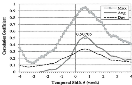
Figure 13. Dependency of temporally-shifted Web Sensor, ws\text{-}doc_{\delta} , using Weblog documents searched by Google on temporal shift \delta for earthquake.
