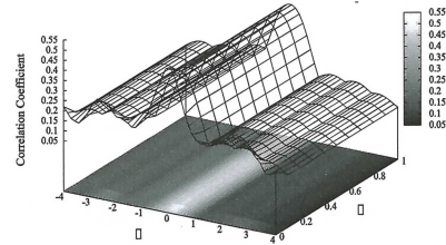
Figure 14. Dependency of combined Web Sensor, ws_{\delta}^{\alpha} , using Web queries and documents on temporal shift \delta and combination param \alpha for rainfall. ( Max 0.53993 when \delta = \pm 0 (week) = \pm 0 (day) and \alpha = 0.00211 )
