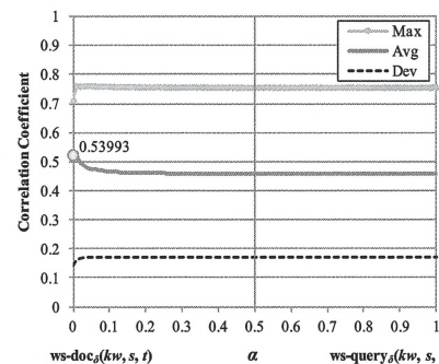
Figure 17. Dependency of combined Web Sensor, ws_{\delta}^{\alpha} , using Web queries and Weblog documents on combination parameter \alpha for rainfall.
