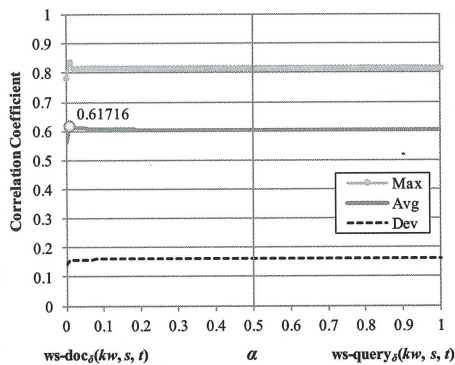
Figure 18. Dependency of combined Web Sensor, ws_{\delta}^{\alpha} , using Web queries and Weblog documents on combination parameter \alpha for snowfall.
