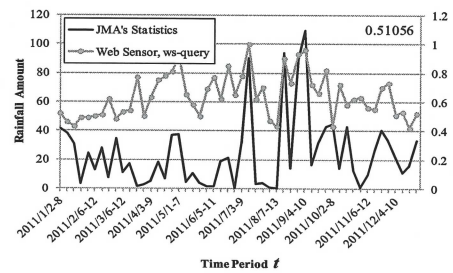
Figure 2. JMA's weekly statistics and Web Sensor's data using Web queries collected by Google Trends for rainfall in Hokkaido prefecture, 2011.
