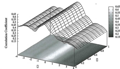
Figure 15. Dependency of combined Web Sensor, ws_{\delta}^{\alpha} , using Web queries and documents on temporal shift \delta and combination param \alpha for snowfall. ( Max 0.61716 when \delta = -1.43 (week) = -1 (day) and \alpha = 0.00907 )
