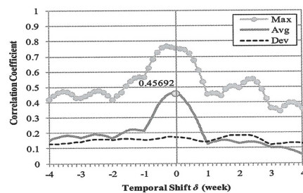
Figure 8. Dependency of temporally-shifted Web Sensor, ws-query δ , using Web queries collected by Google Trends on temporal shift δ for rainfall.
